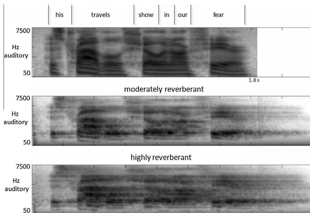
Fig. 2. Auditory spectrograms of the utterance “his travels show in our fear” recorded in near-anechoic conditions (top), then reproduced via loudspeakers and recorded in a 5 × 9 m games room (middle) and a 7 × 3 m bathroom (lower).
